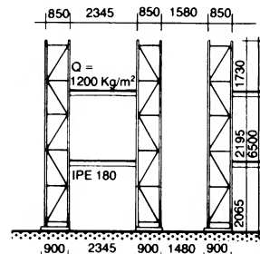
⑨ Section through pallet rack for combined manual operation and operation by stacker (small articles)
